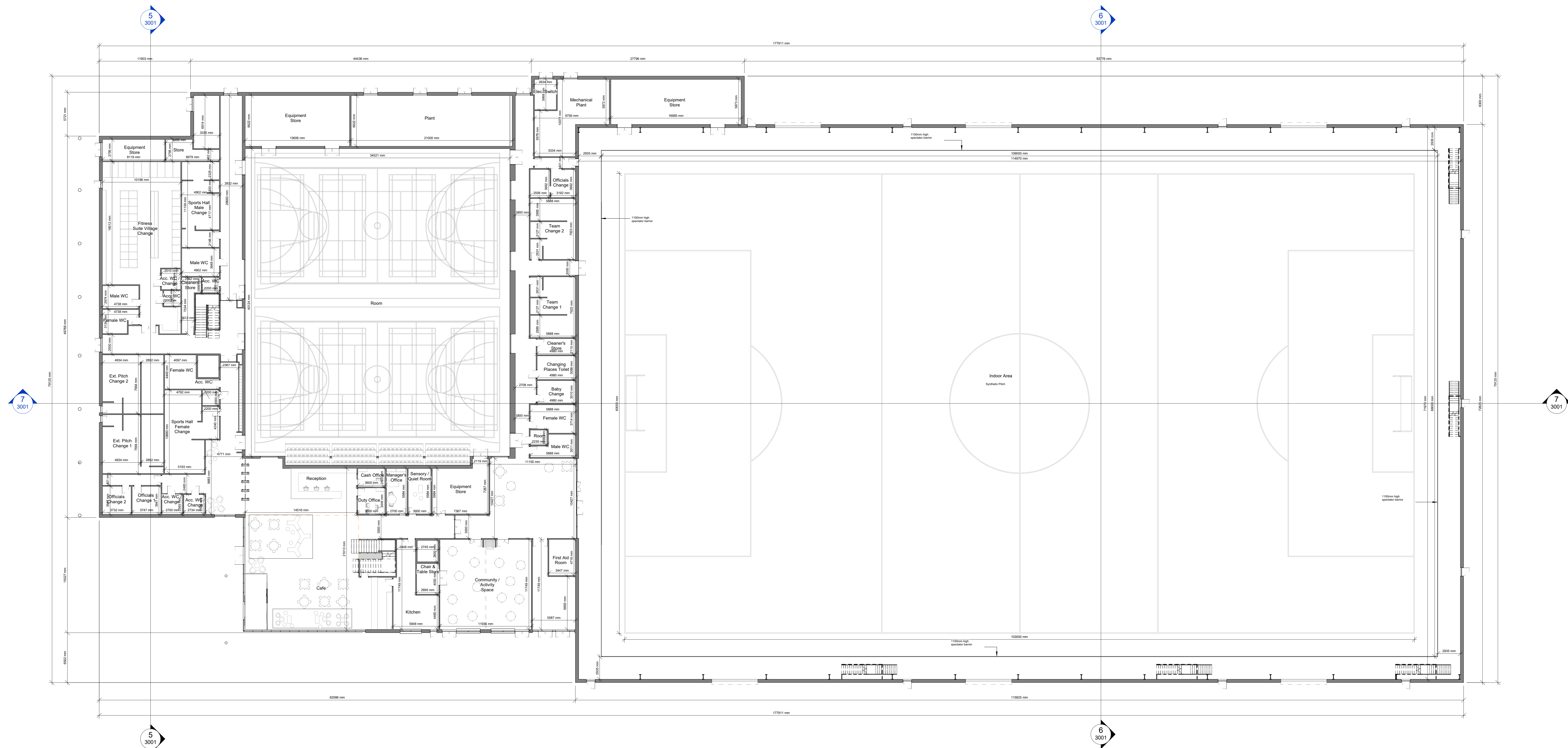
1 Plan - Sports Building - Level 00 Scale: 1 : 200
