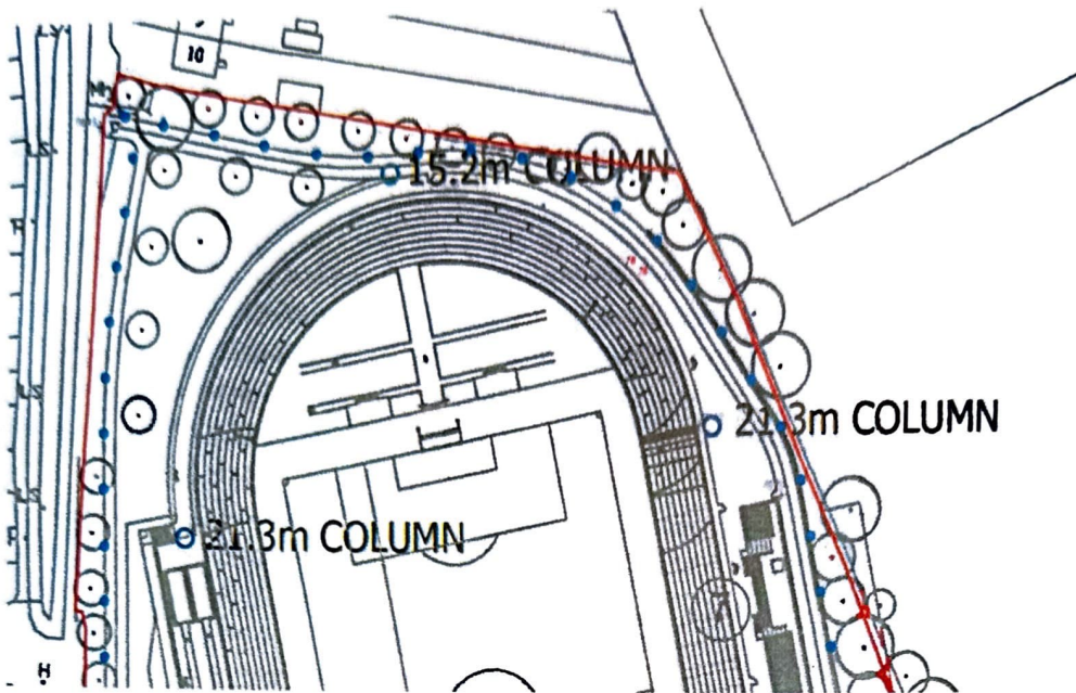
Figure 3 - extract 9955-JCP-ZZ-00-dr-e-63003 - flood light column within 6m of boundary
