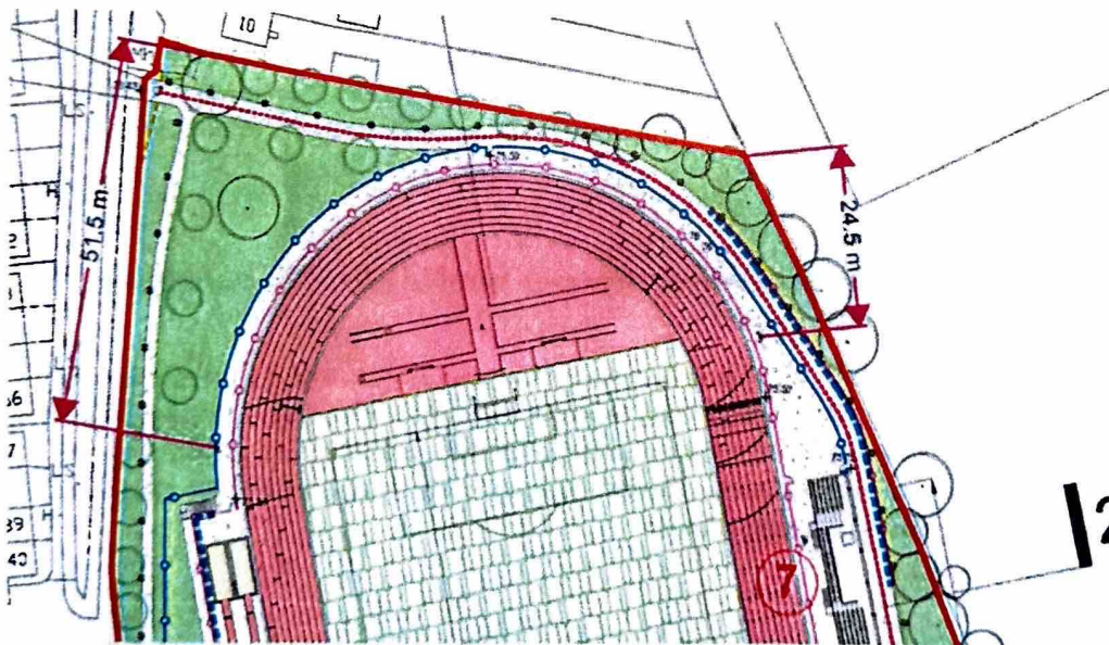
Figure 2 - Extract from A2156-100-10 - Tower flood light locations.
