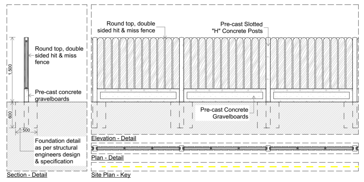
3 Boundary Wall 'A1' 1:50
