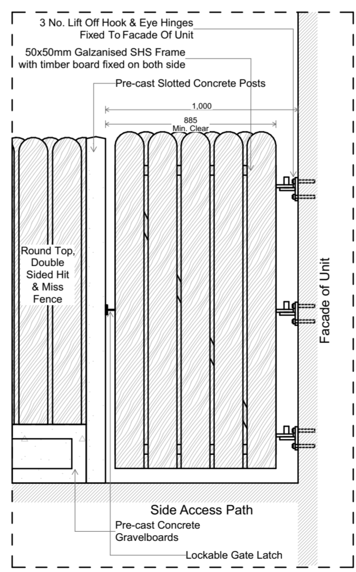
5 Garden Gate Access 1:20
