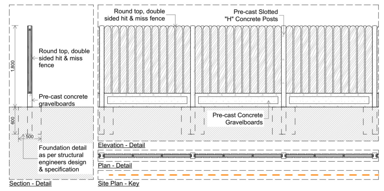
2 Boundary Wall 'A' 1:50
