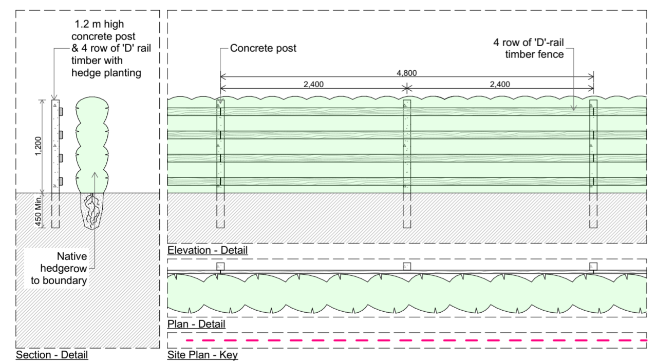
4 Boundary Wall 'D' 1:50
