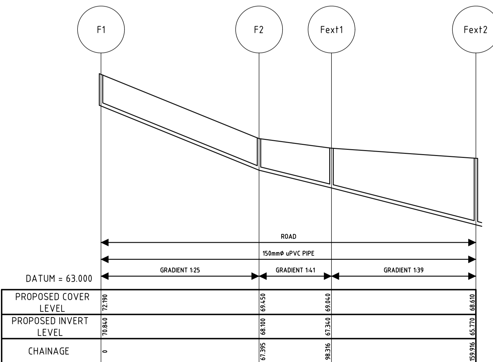
PROPOSED FOUL SEWER SECTIONS F1 - Fext2 HORIZONTAL SCALE 1:1000 VERTICAL SCALE 1:100
