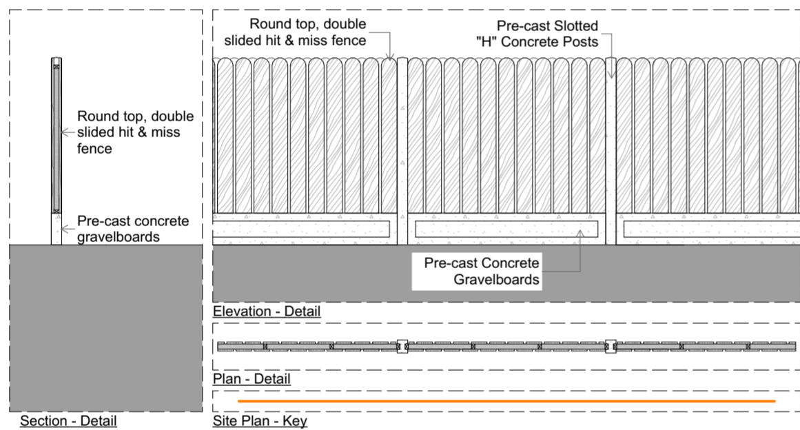
Boundary Wall 'A' 1:50
