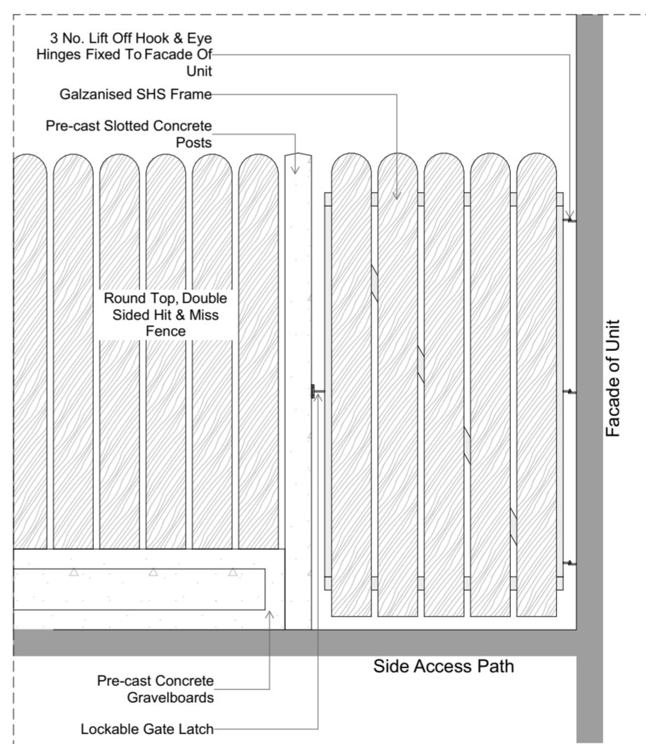
Garden Gate 1:20
