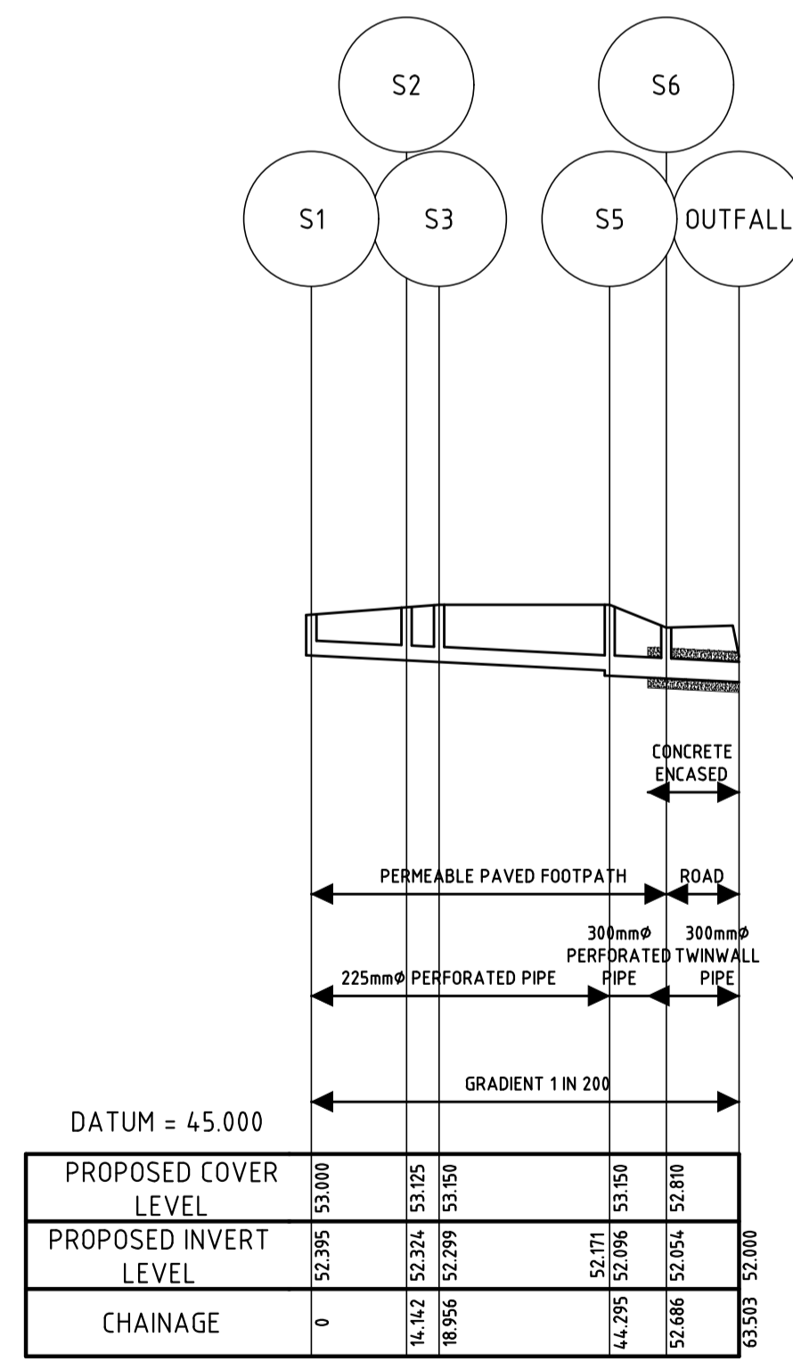
PROPOSED STORM SEWER SECTIONS S1-OUTFALL HORIZONTAL SCALE 1:1000 VERTICAL SCALE 1:100
