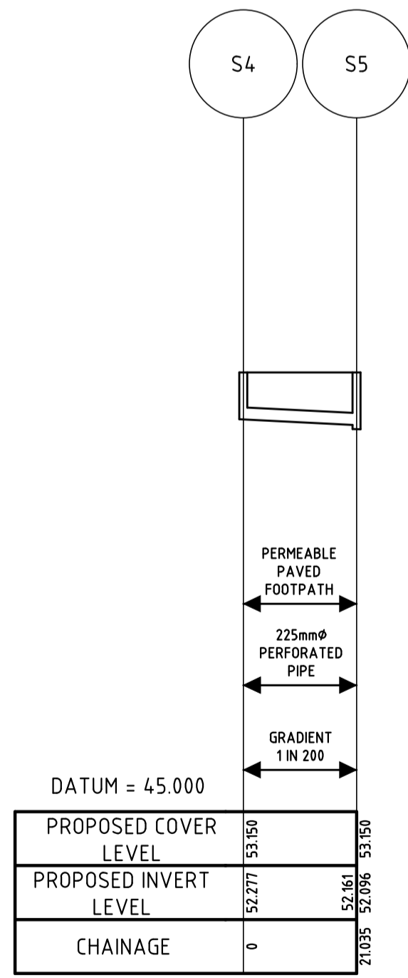
PROPOSED STORM SEWER SECTIONS S4-S5 HORIZONTAL SCALE 1:1000 VERTICAL SCALE 1:100
