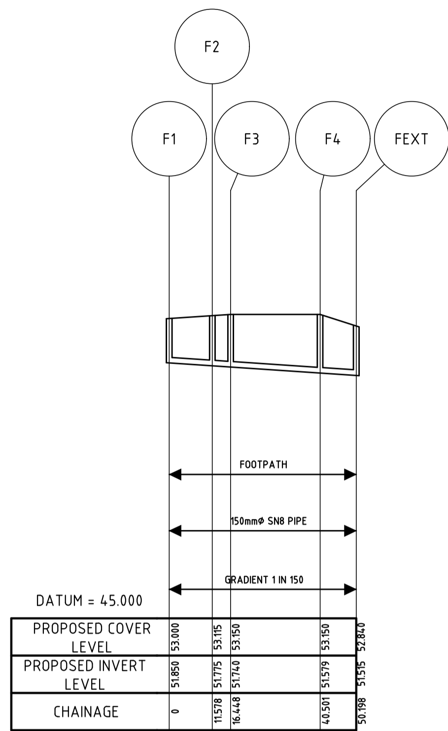
PROPOSED FOUL SEWER SECTIONS F1-FEXT HORIZONTAL SCALE 1:1000 VERTICAL SCALE 1:100
