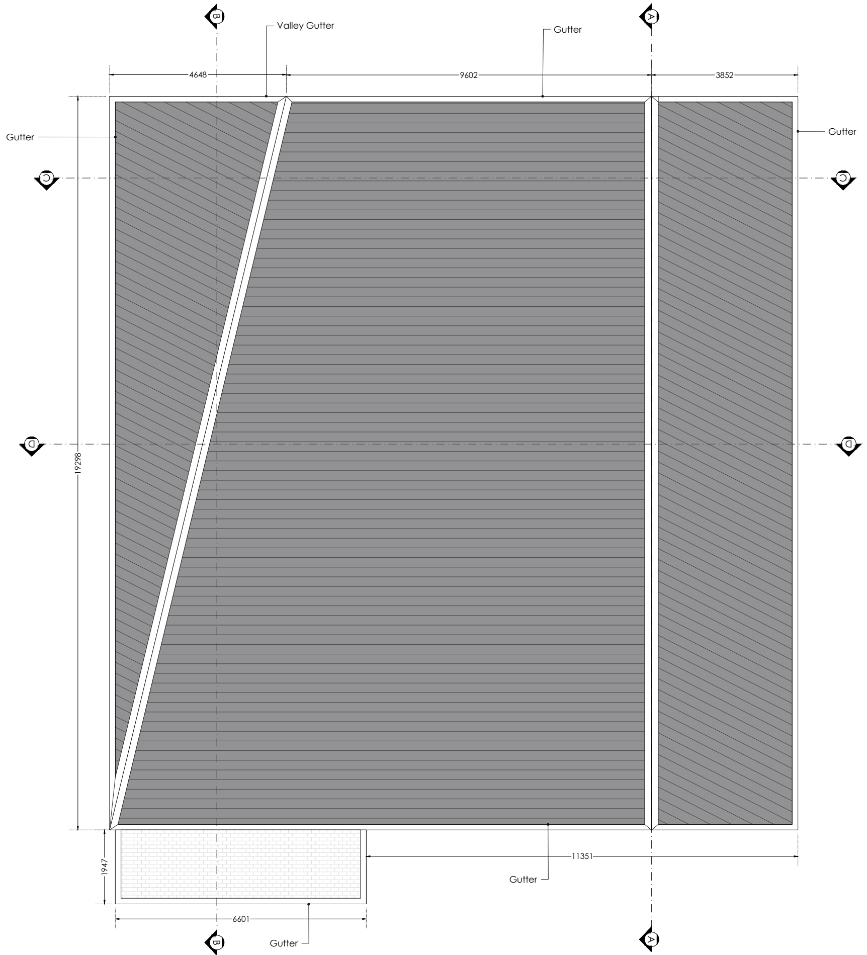
Proposed Roof Floor Plan SCALE 1:100
