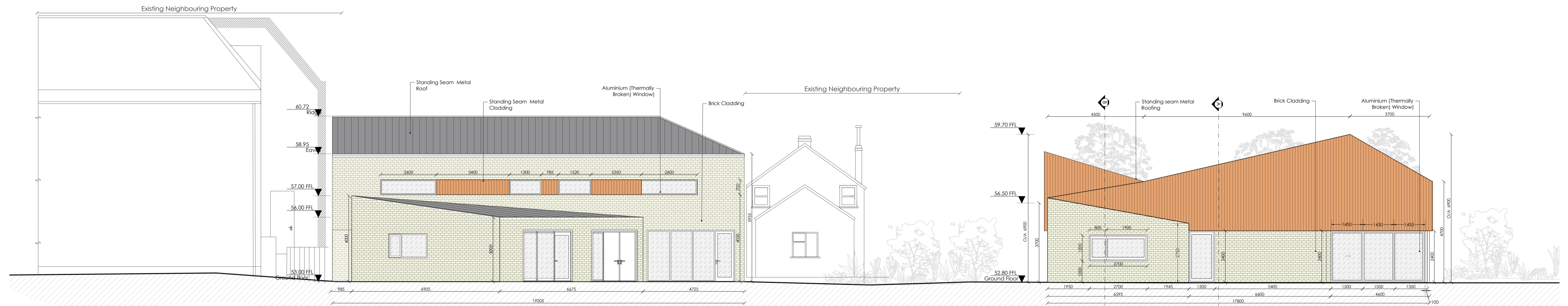
Proposed Rear Street Elevation SCALE 1:100
