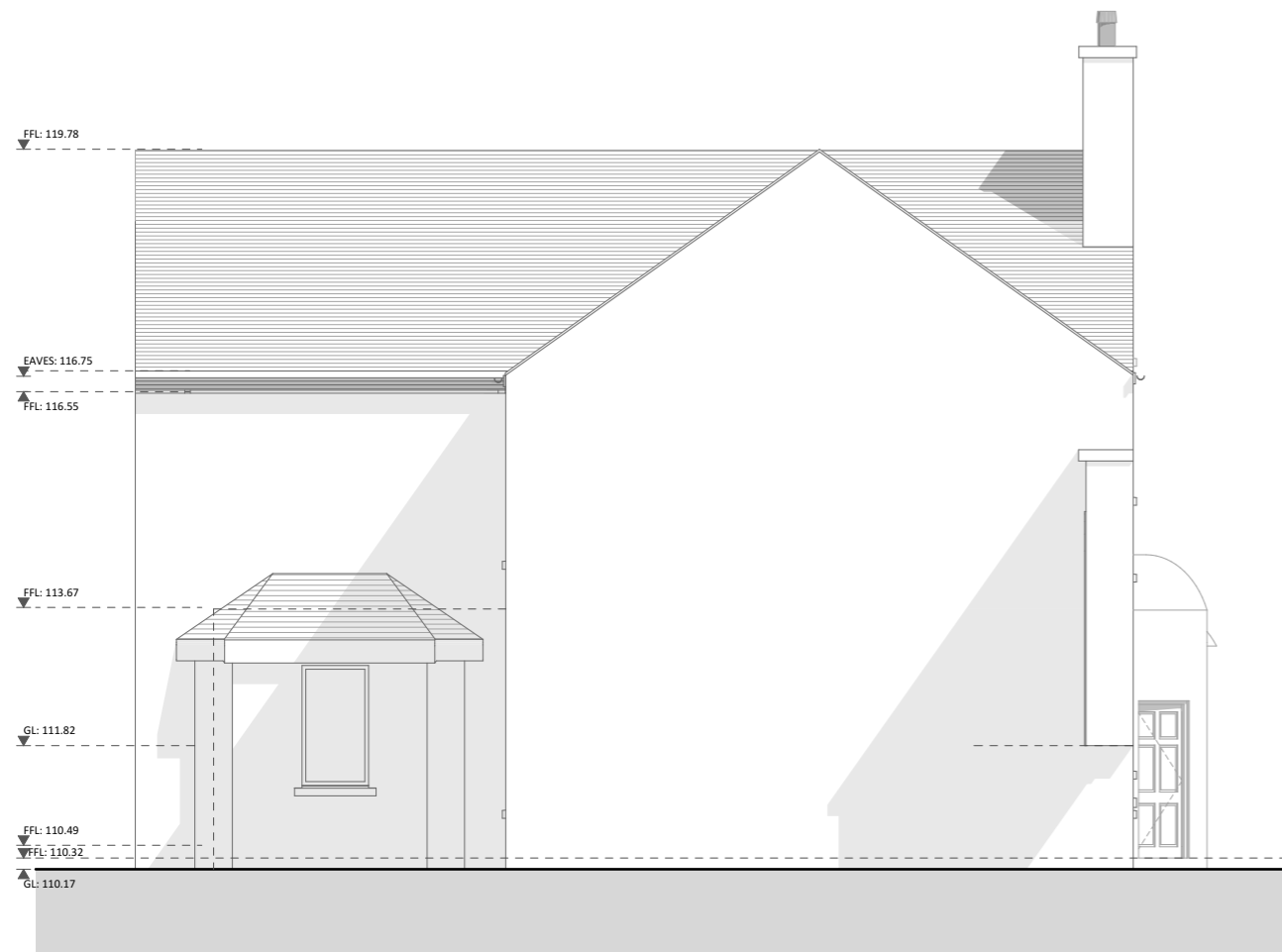
Elevation South 1:100
