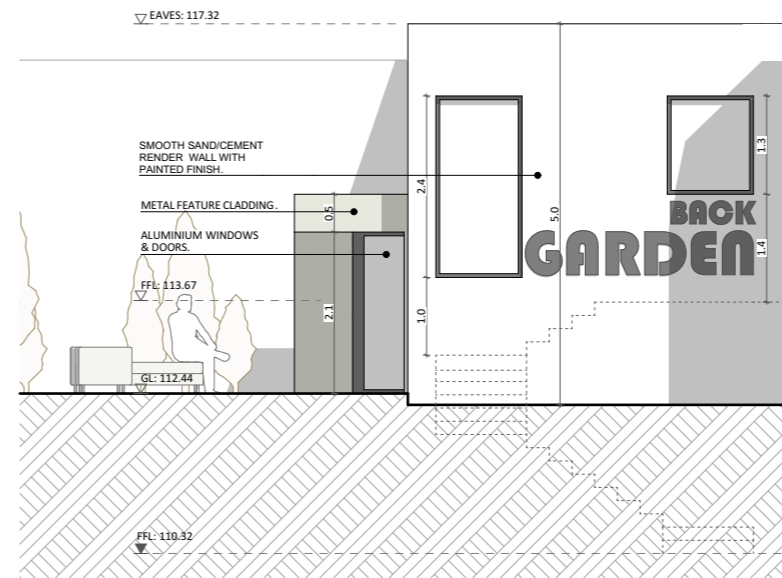
Elevation South - Garden 1:100
