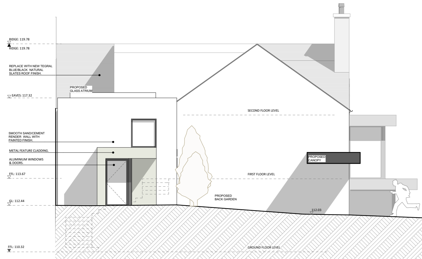
Elevation West 1:100
