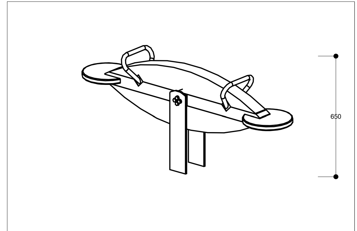
TP09 - Small See Saw - Iso 01 NTS
