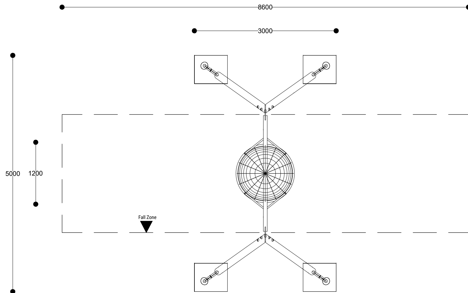
TP01 - Cradle Nest Special - Plan 01 @1:50
