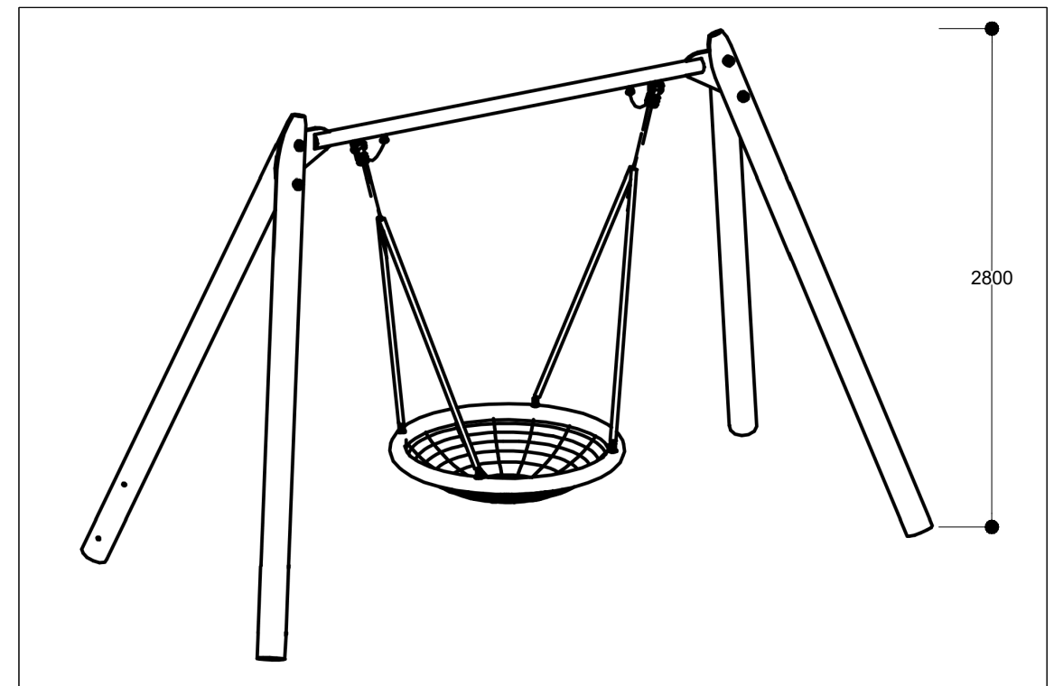
TP01 - Cradle Nest Special - Iso 01 NTS
