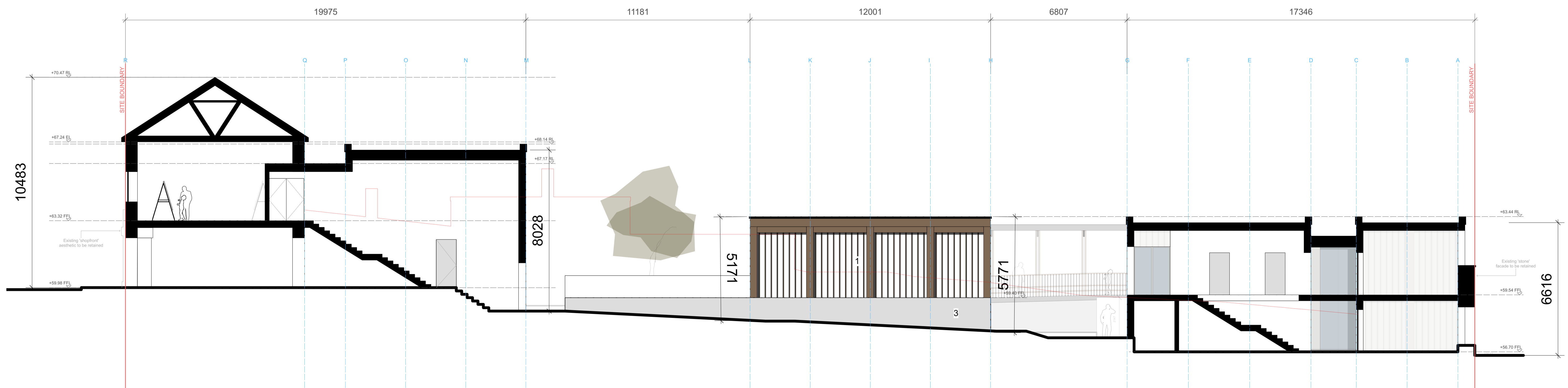
Proposed Site Section 02 Scale: 1:100
