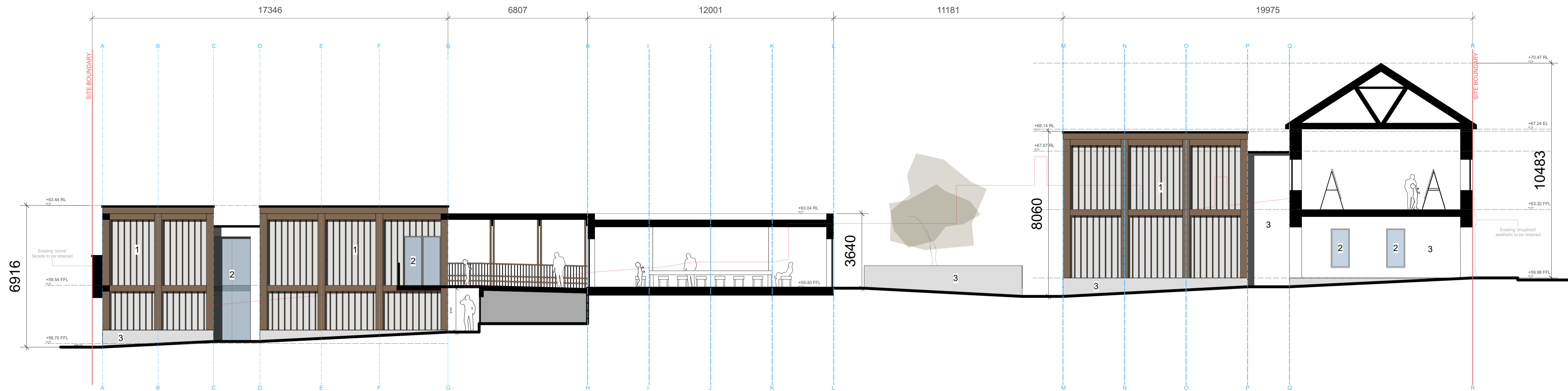
Proposed Site Section 01 Scale: 1:100
