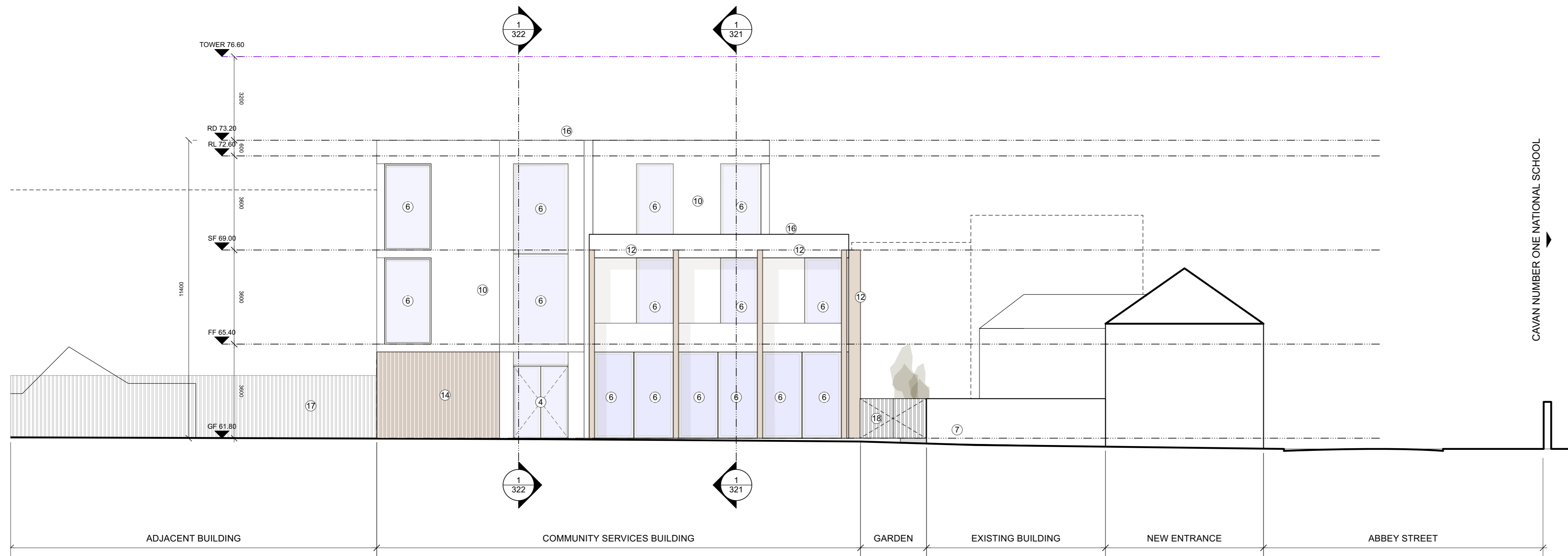
1 Proposed Elevation PP.221 Scale: 1:100
