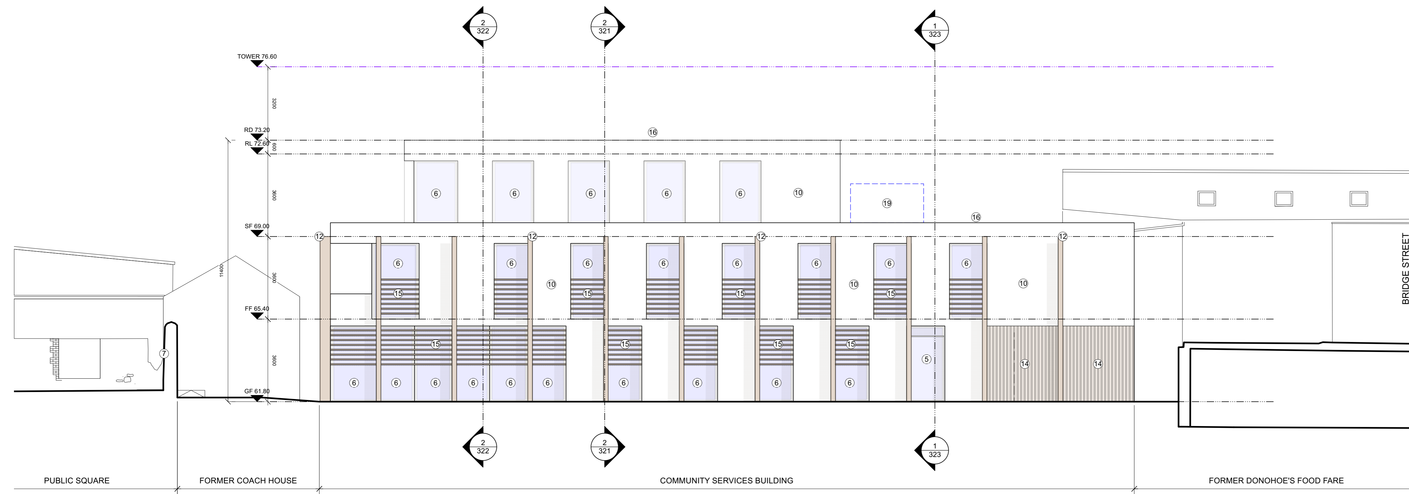
2 Proposed Elevation PP.221 Scale: 1:100
