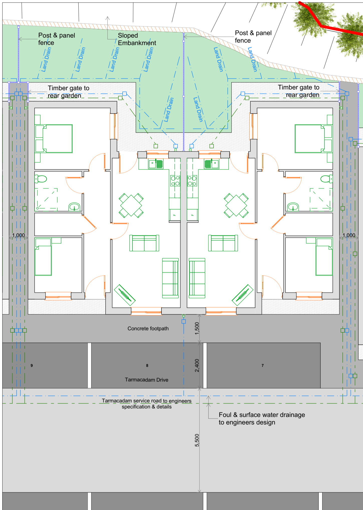
1 Typical Plot Layout (House Type B - Plots 11-12) 1:100
